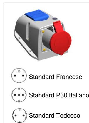
COMBI 16A-32A IP44
