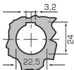
Drilling template (mm)
