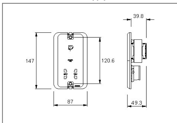
Shaver supply unit
