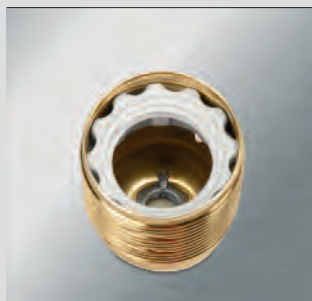
Metal lampholder. Detail of locking screw and earth terminal.
